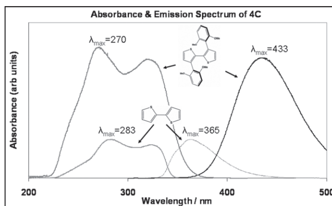
Scheme 1, top: Synthetic pathway for bi-thiophene control compound.
