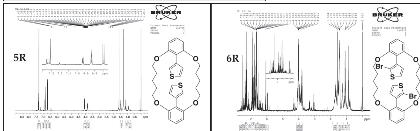
Figure 2, below: H^1 -NMR spectra of 5R and 6R using the same brominating reaction and workup as 2C \rightarrow 3C . Note that 5R/6R and 2C/3C are identical on TLC.
