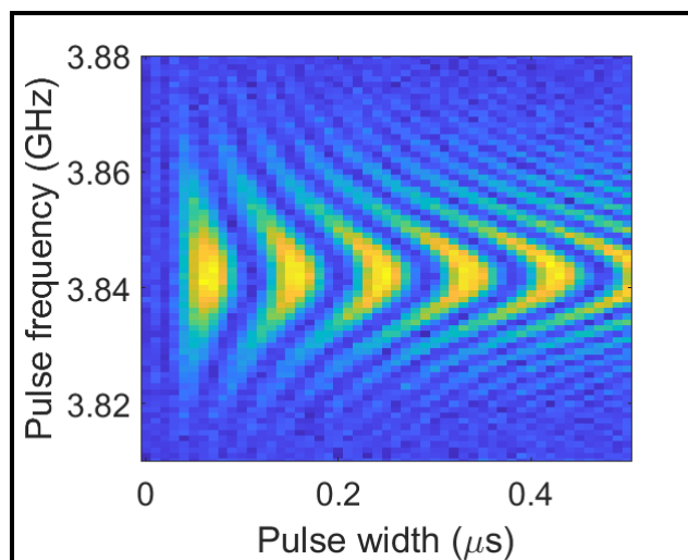
Figure 4: Measurement of Rabi oscillations of transmon qubit coupled to metamaterial ring resonator as a function of microwave drive frequency and pulse duration.
